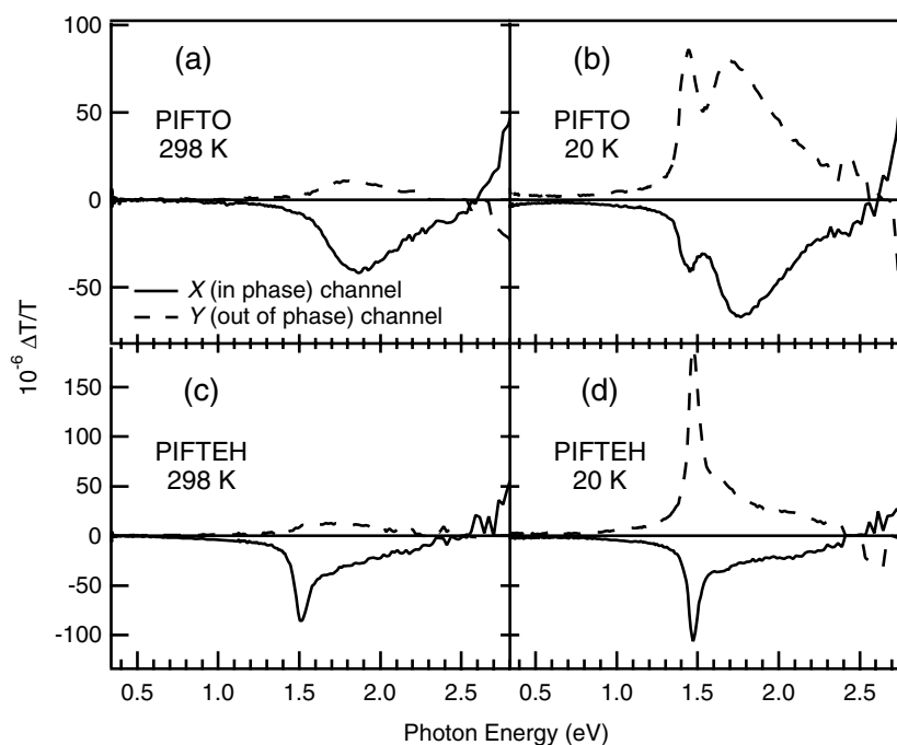
Figure 8. CW-PIA spectra of PIFTO and PIFTEH films at room and low temperatures. The full curves represent the X -channel (in-phase) signal, while the broken curves represent that in the Y channel ( \pi/2 out of phase).
