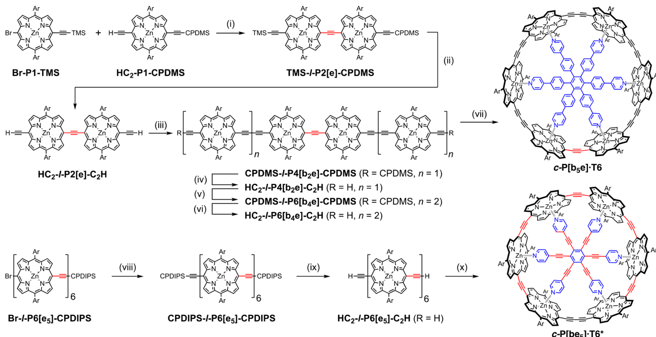
Scheme 1. Synthesis of c\text{-P6}[\text{b}_3\text{e}]\cdot\text{T6} and c\text{-P6}[\text{be}_3]\cdot\text{T6}^* a
