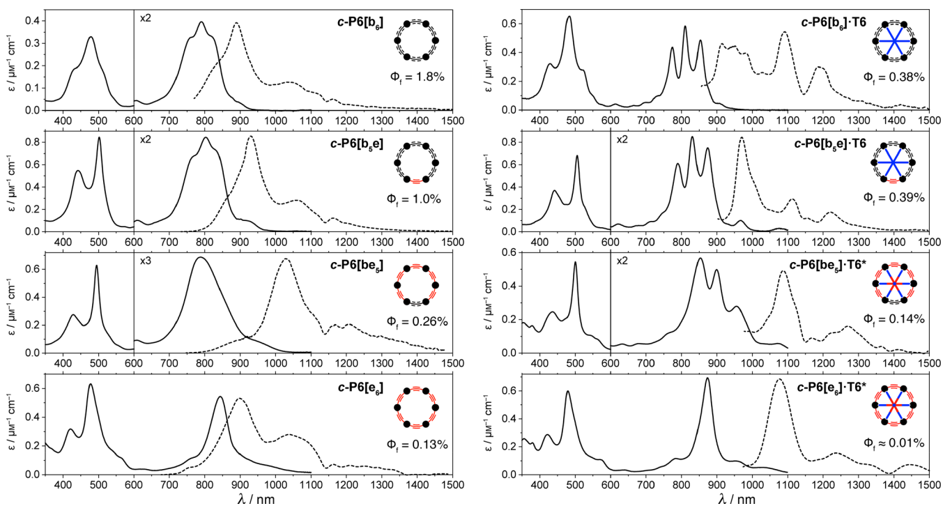
Figure 6. Absorption (black lines) and fluorescence (dashed lines) spectra at 298 K of (left) c-P6[b 6 ], c-P6[b 3 e], c-P6[be 5 ], c-P6[e 6 ] in toluene containing 1% pyridine and (right) c-P6[b 6 ]-T6, c-P6[b 3 e]-T6, c-P6[be 5 ]-T6*, and c-P6[e 6 ]-T6* in toluene. Fluorescence quantum yields ( \Phi_f ) are given in %. The dip in the fluorescence spectra at around 1140 nm is due to absorption by the solvent.
