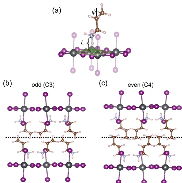
Fig. 5 DFT-derived structures of 2D perovskites. (a) Illustration of the vertical distance L of the \text{N}-\text{PbI}_x plane and the angle \psi between the horizontal plane and the tail of the ligands. Examples for packing of the organic ligands within the inorganic lattice for (b) odd and (c) even numbers of carbon atoms in the spacer cation.
