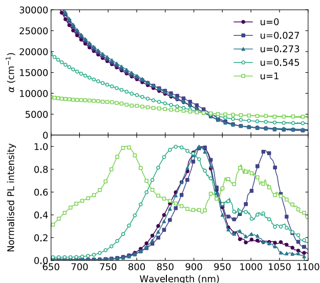
Figure 2. Absorption coefficient, \alpha , (top) and normalized PL (bottom) spectra near the absorption edge of \text{FA}_{1-x}\text{Cs}_x\text{Sn}_{1-y}\text{Pb}_y\text{I}_3 perovskite thin films on quartz. PL was obtained using a 400 nm continuous wave laser with an intensity of 1.27 \text{ W/cm}^2 for excitation. The legend indicates different values of the \text{SnF}_2 fraction, u . Markers in the absorption spectra indicate every 75th data point, whereas markers in the PL spectra indicate every 10th data point. \alpha = A/d , where absorbance A = -\ln(T/(1 - R)) , d is film thickness, T is transmittance, and R is reflectance.
